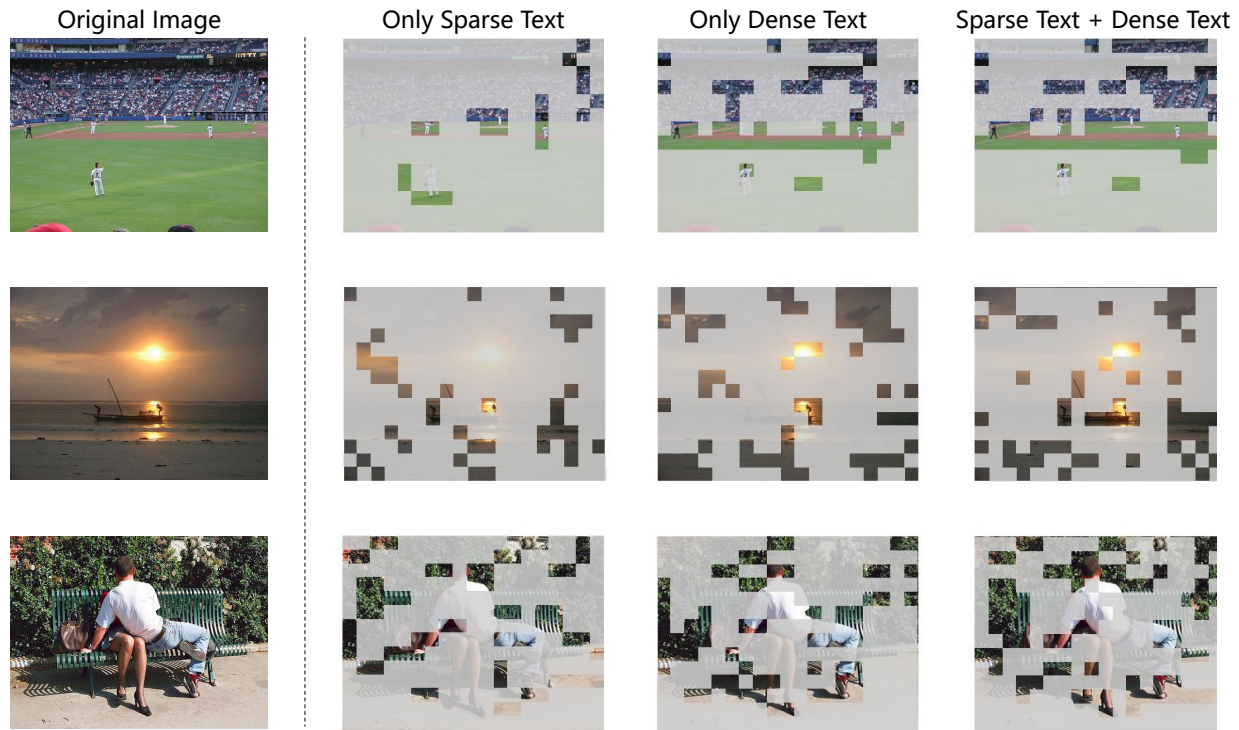
Figure 5. The visualization of visual patch selection with different combinations of sparse text and dense text.
